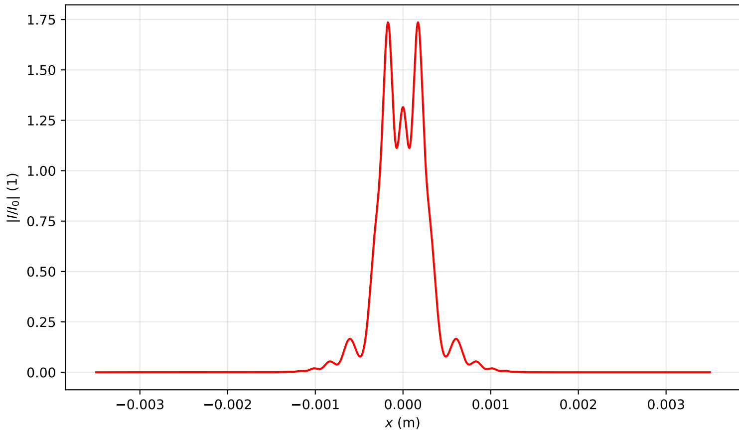
Intensity profile I(x, y = 0, z = 0.716)/I_0 , P_{in}=4.5P_{cr} , artificial time
